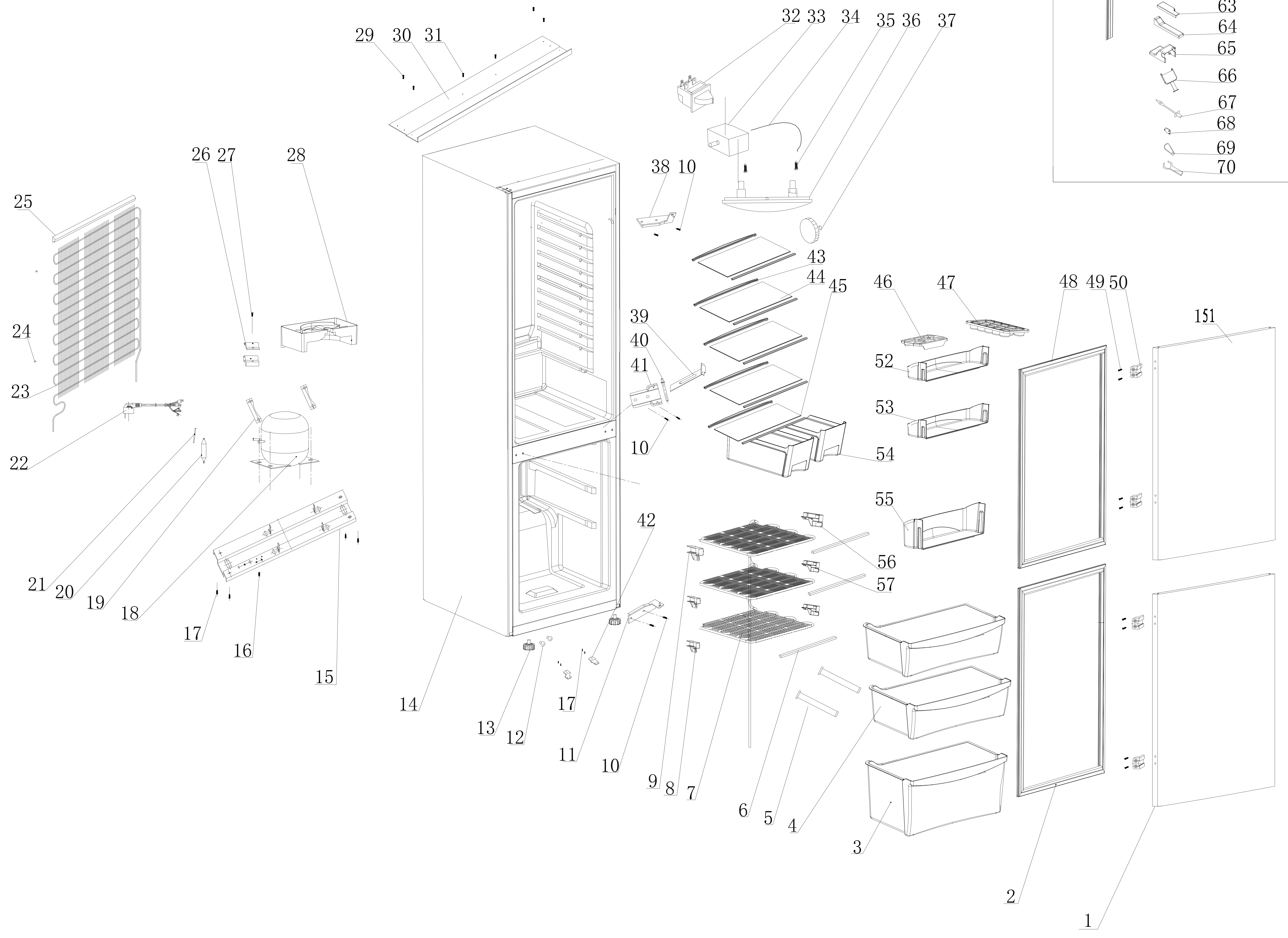
TRF-32BIAA Exploded View
